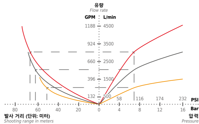
TORNADOMATIC 3000 노즐 DIFFUSER TORNADOMATIC 3000 AUTOKADOR 5000 노즐 DIFFUSER AUTOKADOR 5000
